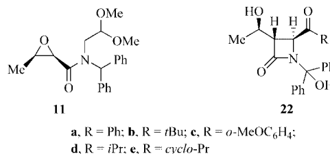
Figure 3. Synthetic intermediates 11 and 22a–e .
