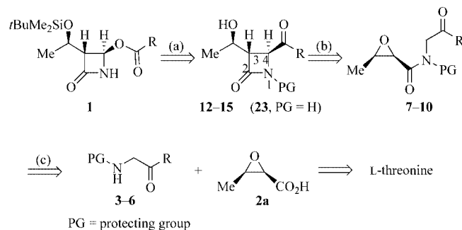
Scheme 1. Retrosynthetic scheme: (a)–(c) see text.
