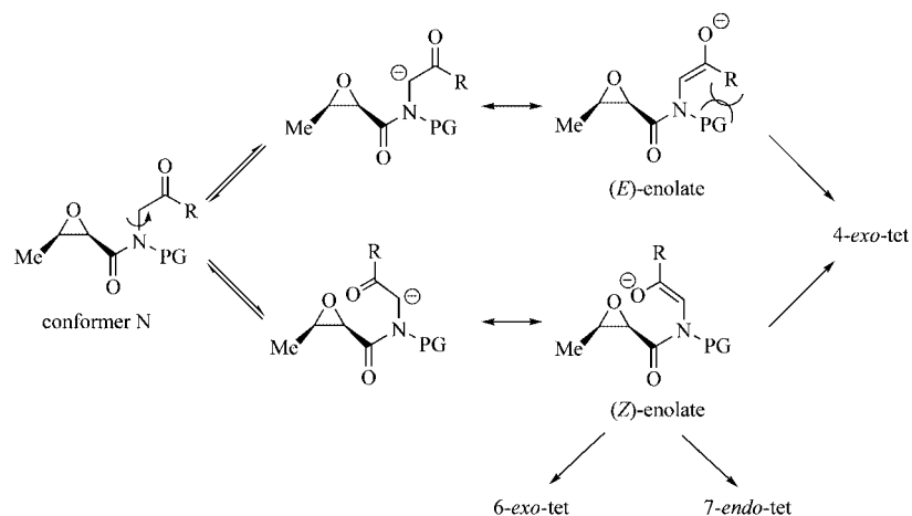
Scheme 3. Cyclization processes (the process is named exo when the C–C bond of the epoxide is outside the formed cycle and endo when the C–C bond of the epoxide is inside the formed cycle).
