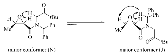
Figure 1. Rotamers of 8b with NOESY correlations indicated.
