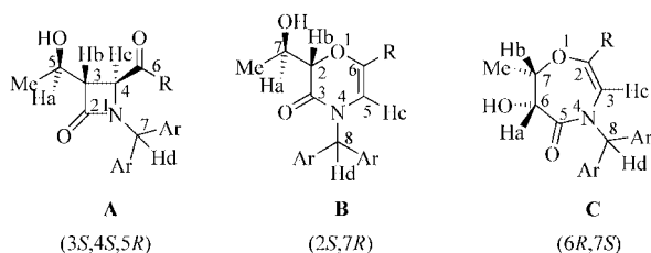
Figure 2. Atom numbering considered in Tables 4–6.
