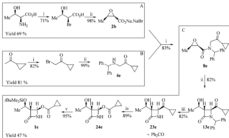
Scheme 5. Part A: i: \text{NaNO}_2 , \text{KBr} , \text{H}_2\text{SO}_4/\text{H}_2\text{O} , -10\text{ }^\circ\text{C} to 20\text{ }^\circ\text{C} , 3 h; ii: \text{NaOH} , \text{H}_2\text{O} , -10\text{ }^\circ\text{C} to 20\text{ }^\circ\text{C} , 18 h. Part B: i: \text{Br}_2 , \text{MeOH} , 0\text{ }^\circ\text{C} to 20\text{ }^\circ\text{C} ; ii: \text{K}_2\text{CO}_3 , \text{KI} , \text{Ph}_2\text{CHNH}_2 , \text{DMF} , 20\text{ }^\circ\text{C} . Part C: i: (\text{COCl})_2 , \text{THF} , -5\text{ }^\circ\text{C} , 2 h, then pyridine, 2 h, 20\text{ }^\circ\text{C} ; ii: \text{LiHMDS} , \text{THF} , 0\text{ }^\circ\text{C} , 3 h; iii: \text{NBS} , \text{Br}_2 (catal.), \text{CH}_2\text{Cl}_2/\text{H}_2\text{O} , h\nu , 20\text{ }^\circ\text{C} , 15 h, then \text{PTSA} , \text{acetone}/\text{H}_2\text{O} , 20\text{ }^\circ\text{C} , 18 h; iv: m\text{CPBA} , \text{CH}_2\text{Cl}_2 , 20\text{ }^\circ\text{C} , 18 h; v: \text{TBDMSCl} , \text{imidazole} , \text{DMF} , 20\text{ }^\circ\text{C} , 48 h.
