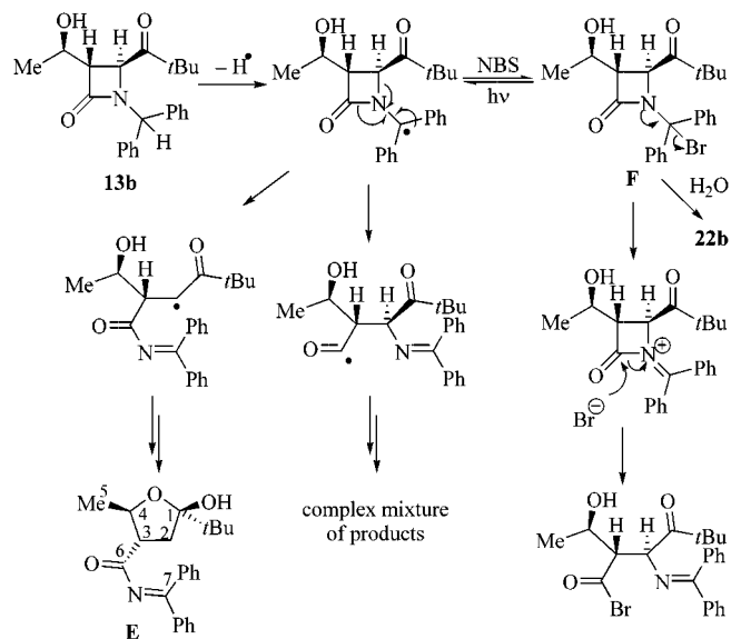
Scheme 4. Postulated routes for the azetidinone degradation.
