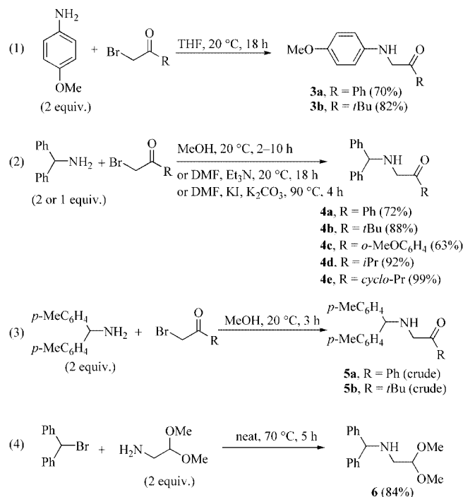
Scheme 2. Synthesis of \alpha -amino ketone reagents.
